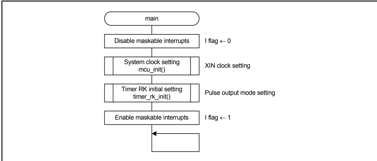
Figure 4.2 Main Processing
