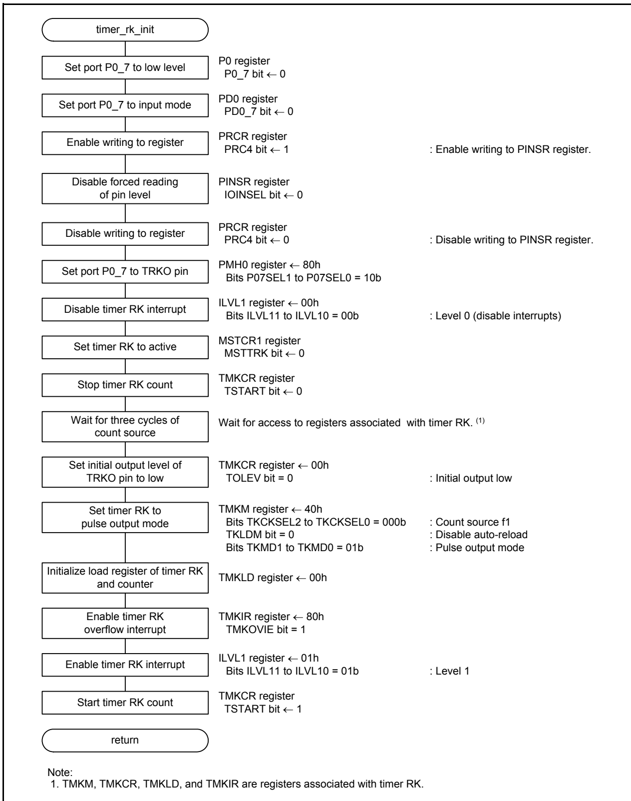
Figure 4.4 Timer RK Initial Setting
