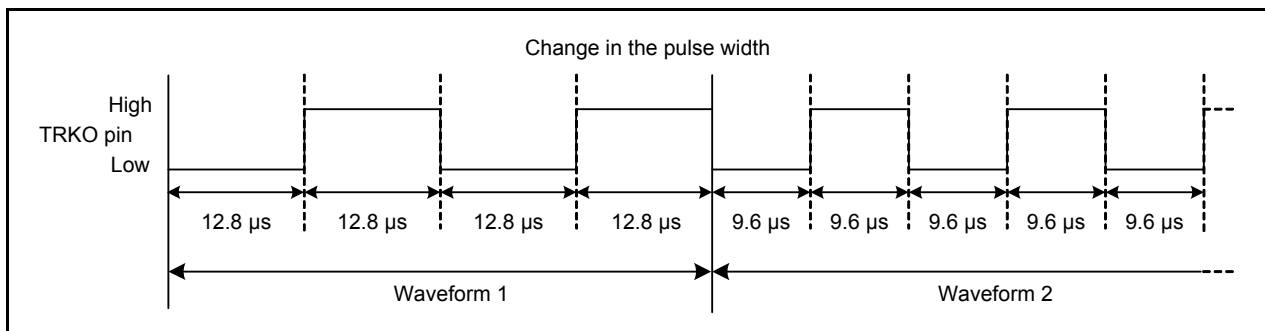
Figure 1.1 Output Waveform
