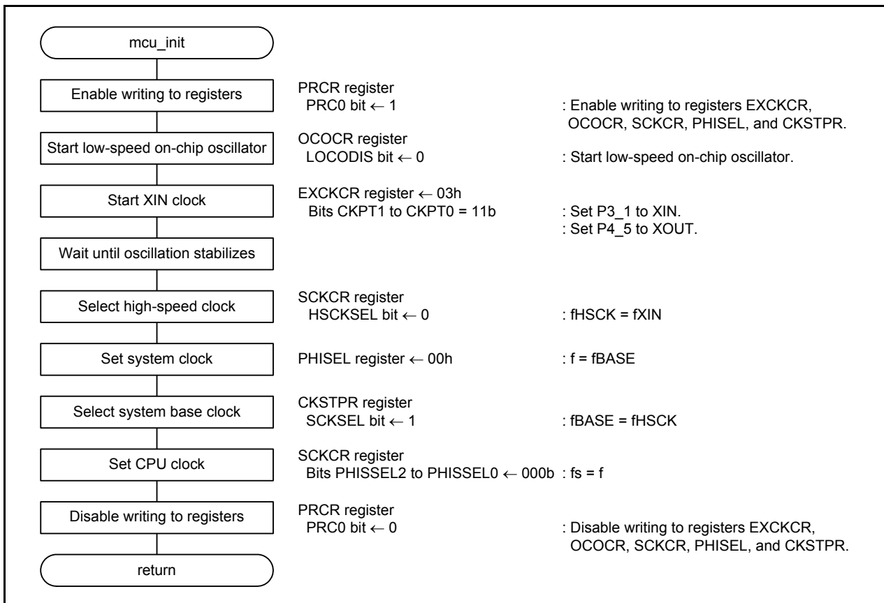
Figure 4.3 System Clock Setting
