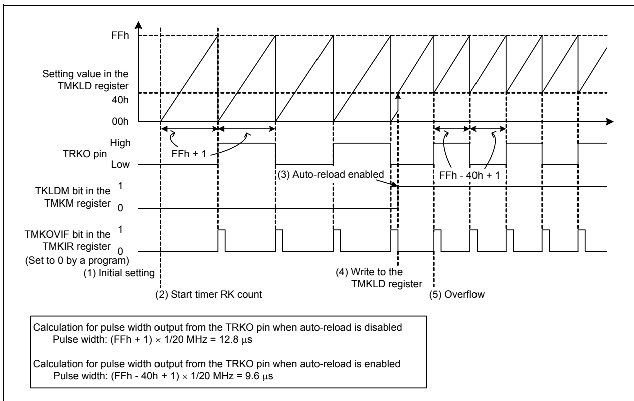
Figure 4.1 Timing Diagram
