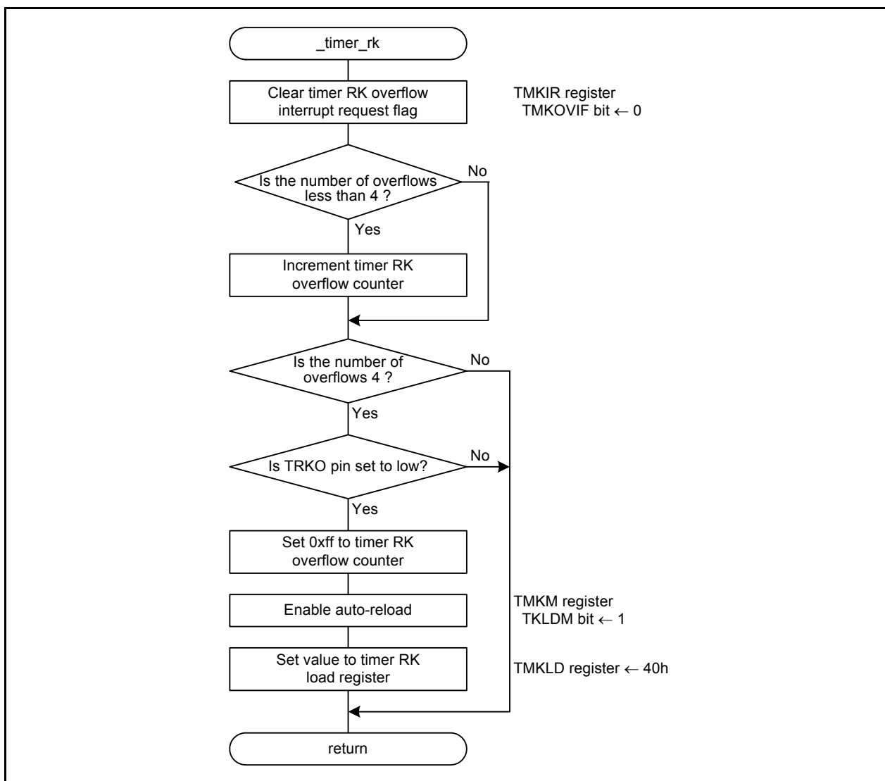
Figure 4.5 Timer RK Interrupt Handling
