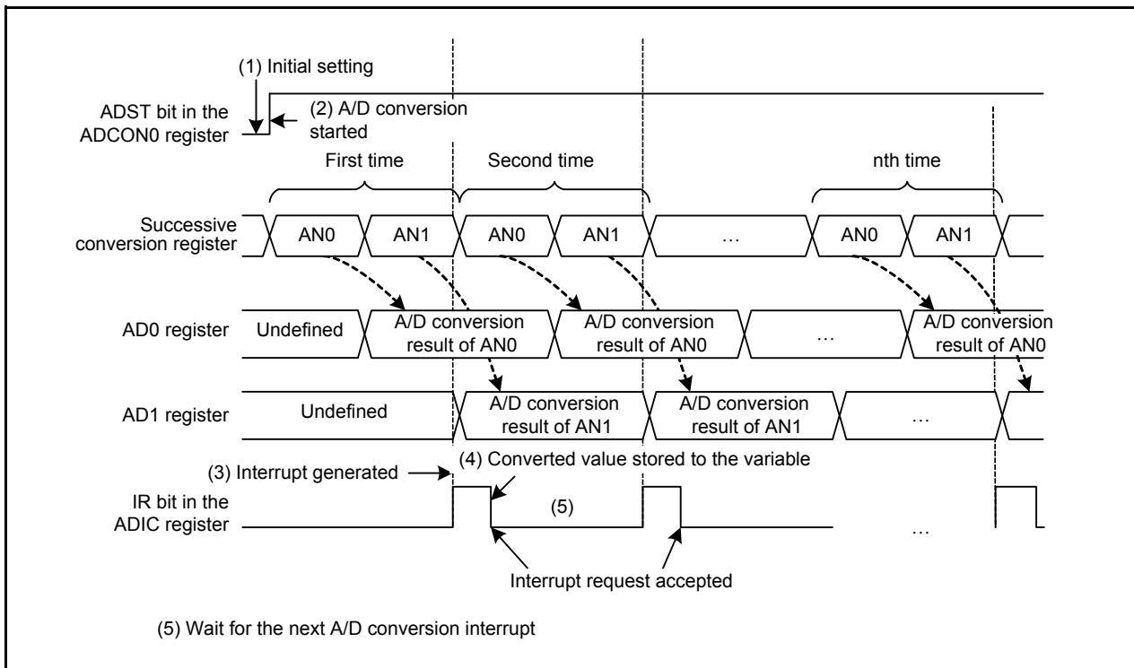
Figure 4.1 Timing Diagram in Repeat Sweep Mode
