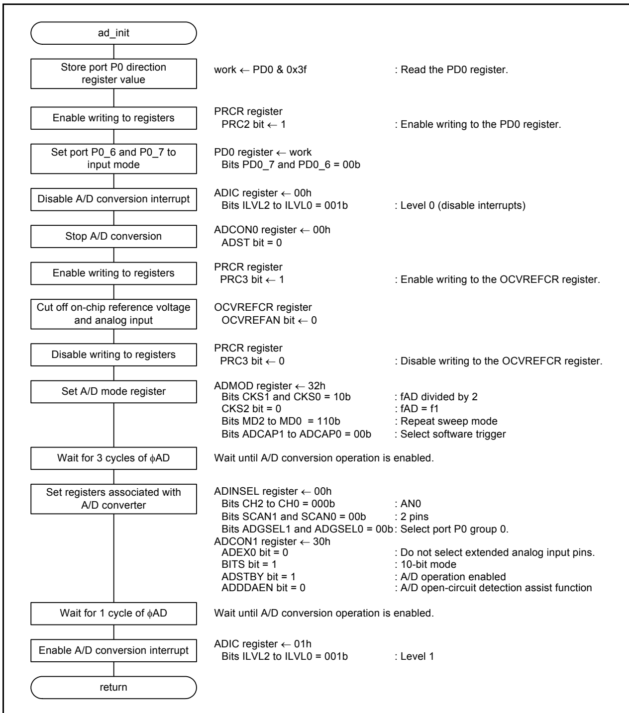
Figure 4.4 Initial Setting of A/D Converter
