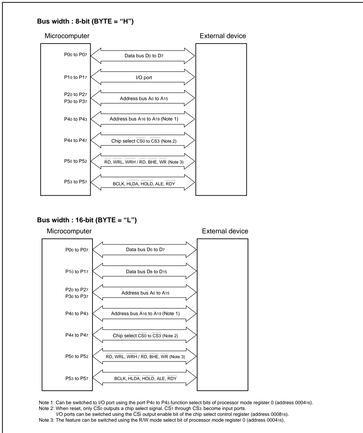
Figure 3.2.1. Level of BYTE pin and external data bus width
