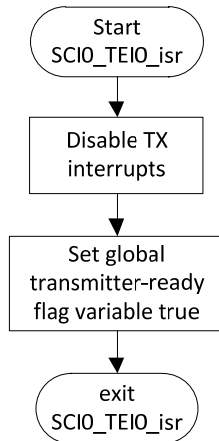
Figure 5. Transmit Completed interrupt service routine flow diagram.
