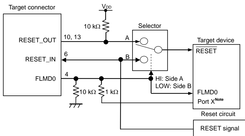
Figure 2-12. Circuit Connection for Automatically Switching Reset Signal with Selector Logic (When Using Flash Self Programming)
