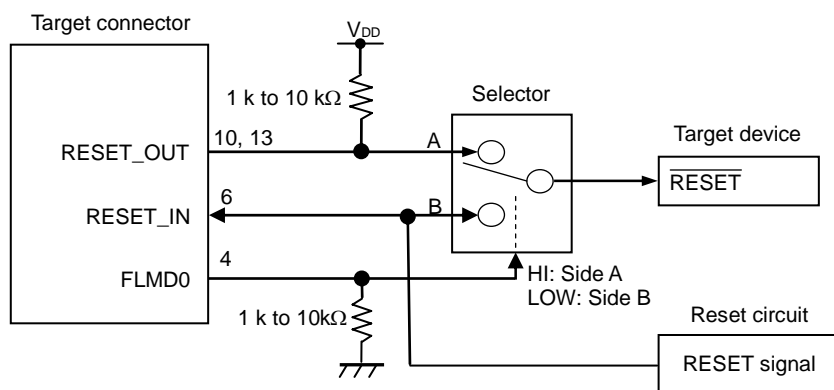
Figure 2-11. Circuit Connection for Automatically Switching Reset Signal with Selector Logic (When Not Using Flash Self Programming)
