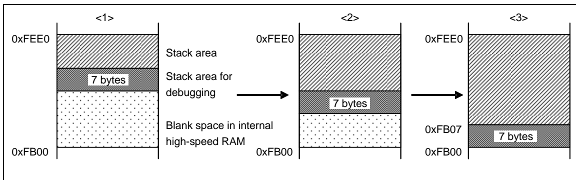
Figure 2-22. Change in Address of Stack Area for Debugging
