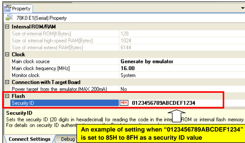
Figure 2-21. Security ID Setting
