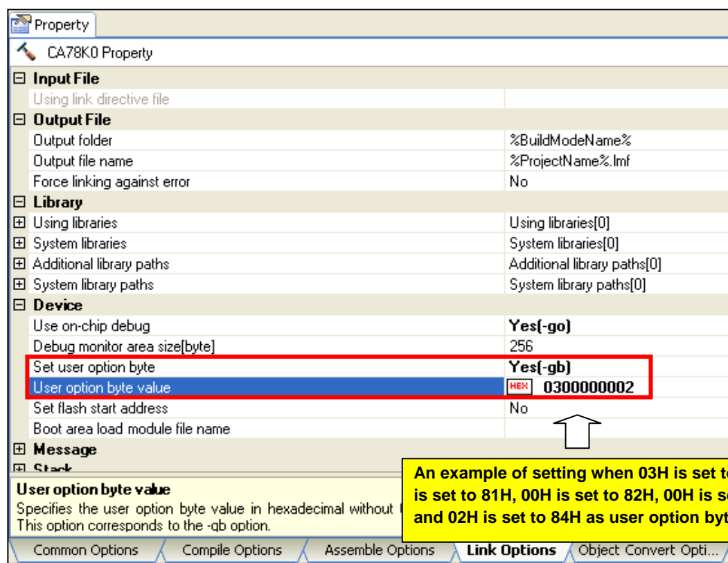
Figure 2-20. User Option Byte Setting
