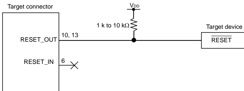
Figure 2-14. Circuit Connection for the Case Where Target Device Is Only Reset via POC
