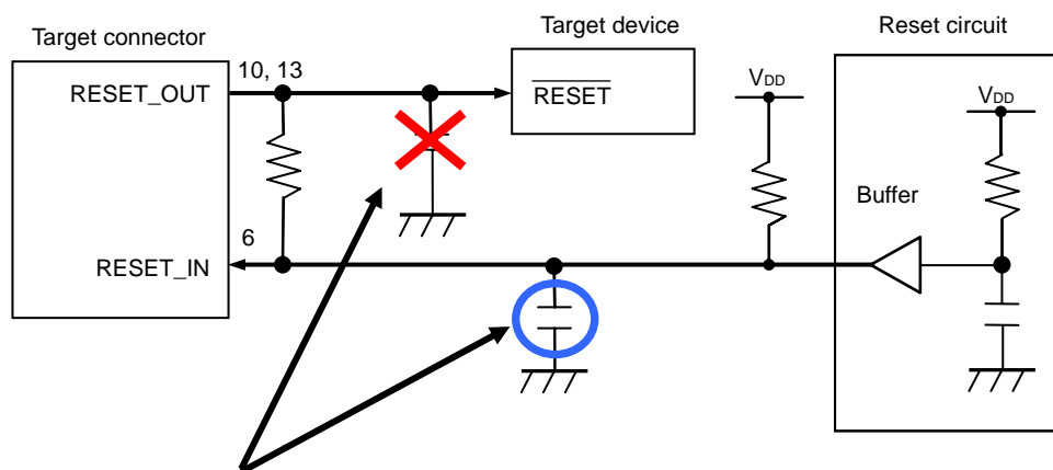
Figure 2-8. Cautions for Using RESET_OUT Pin
