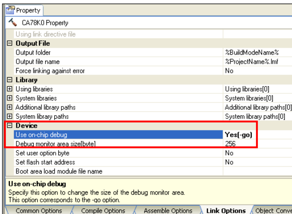
Figure 2-19. Link Option Setting (Debug Monitor Area)
