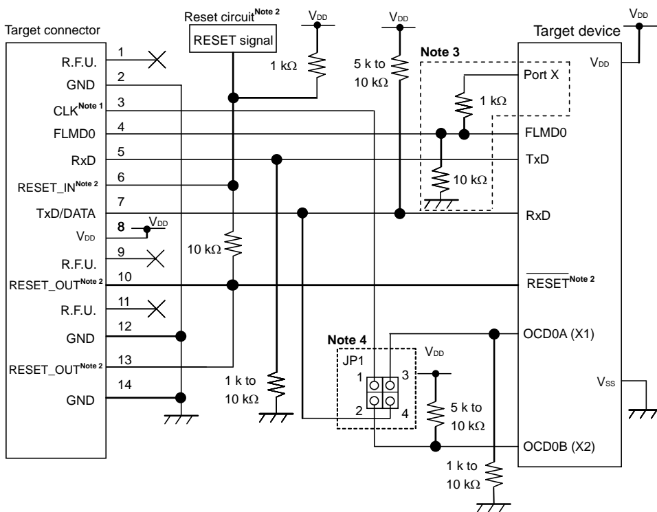
Figure 2-4. Using One Connector for Both Debugging and Programming (OCD0A, OCD0B Communication)
