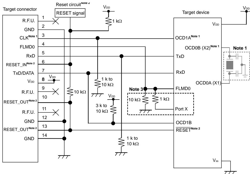
Figure 2-5. Using One Connector for Both Debugging and Programming (OCD1A, OCD1B Communication)
