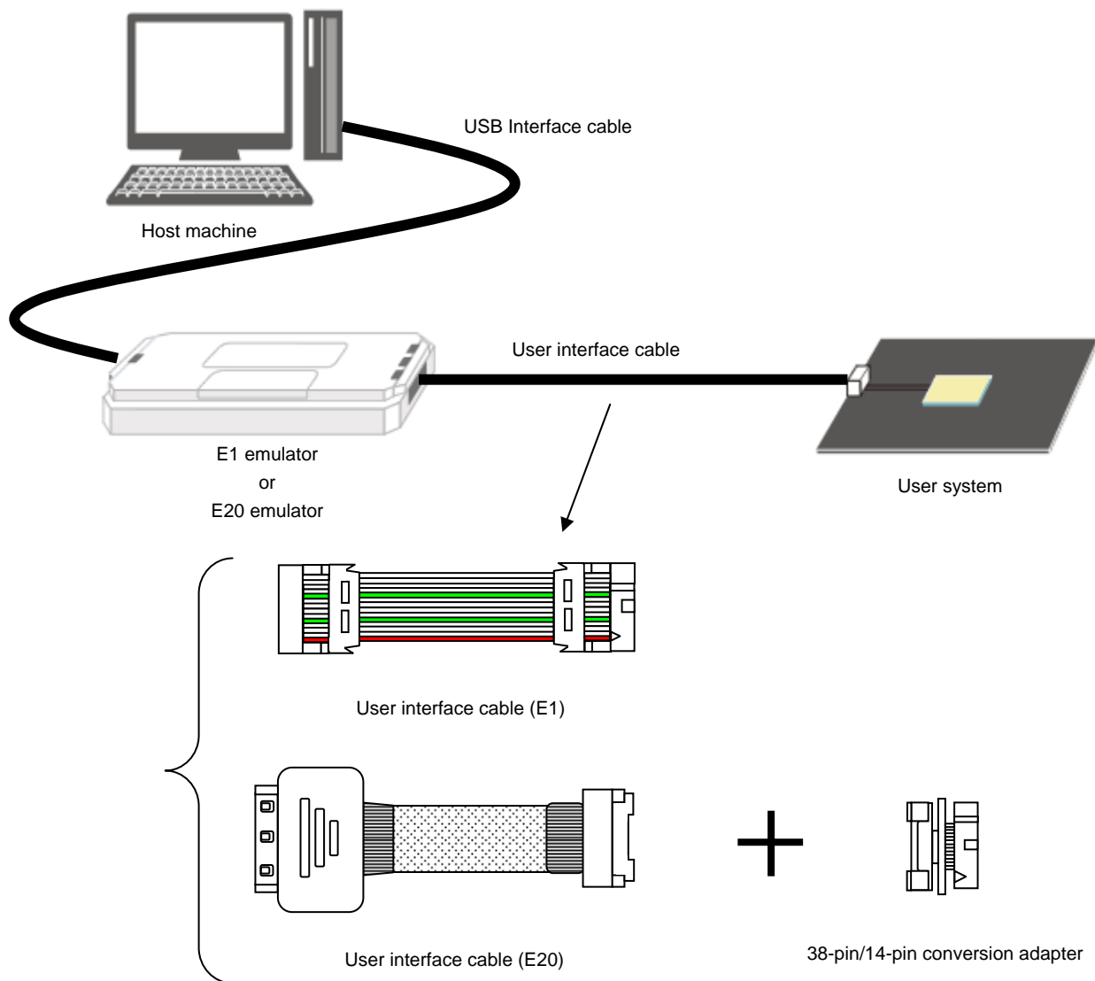
Figure 2-2. Connection Diagram of E1/E20
