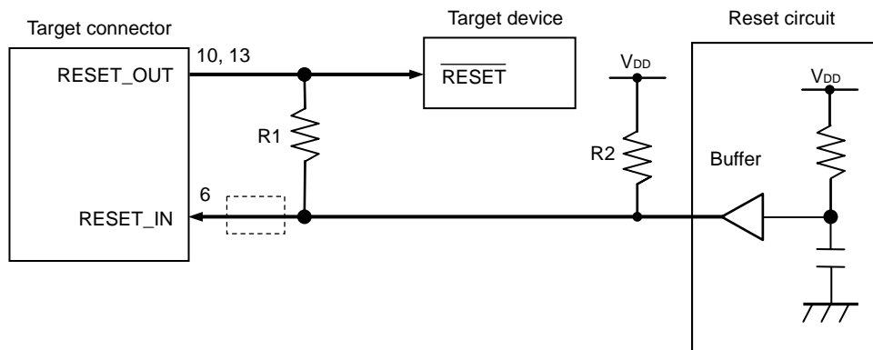
Figure 2-9. Circuit Connection with Reset Circuit That Contains Buffer
