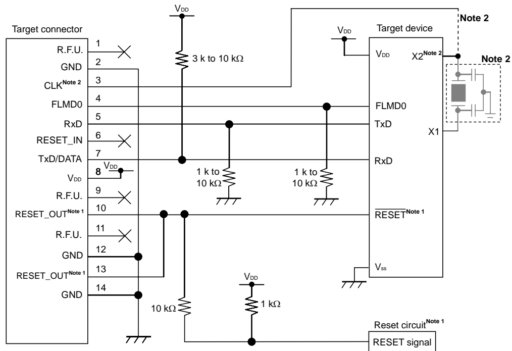
Figure 2-7. Only Programming Is Performed
