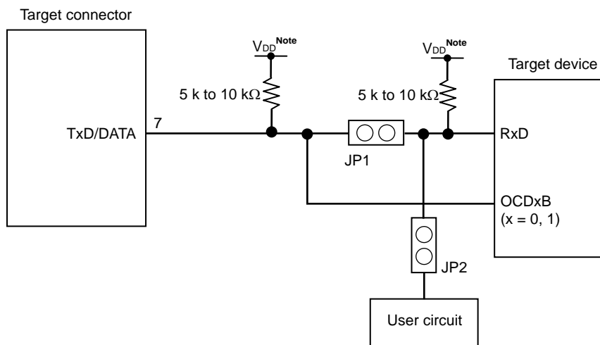
Figure 2-15. Example of Circuit When User Circuit Is Connected to RxD Pin of Target Device
