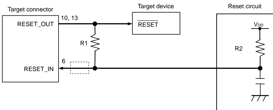
Figure 2-10. Circuit Connection with Reset Circuit That Contains No Buffers
