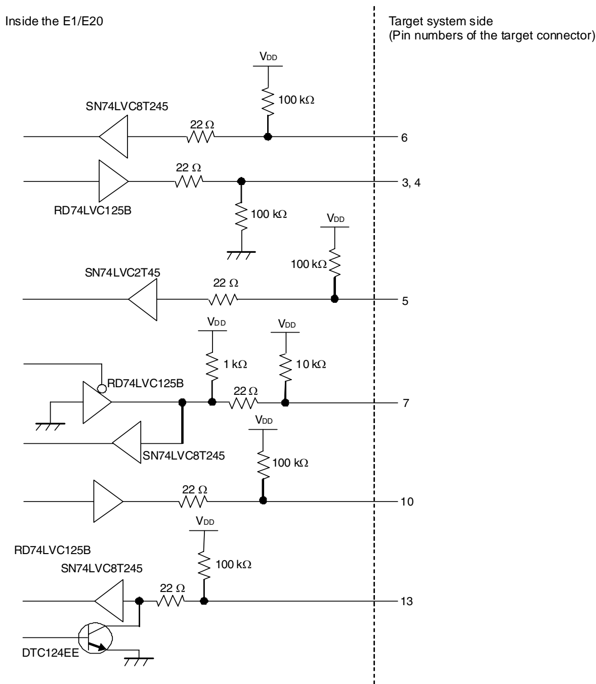
Figure A-1. E1/E20 Equivalent Circuit
