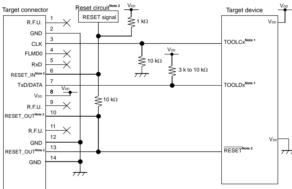
Figure 2-3. Using One Connector for Both Debugging and Programming (TOOLCx/TOOLDx Communication x = 0, 1)
