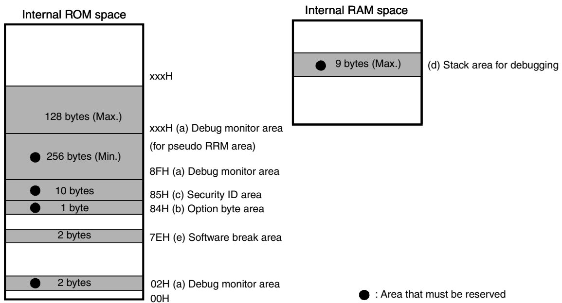
Figure 2-18. Reserved Area Used by E1/E20
