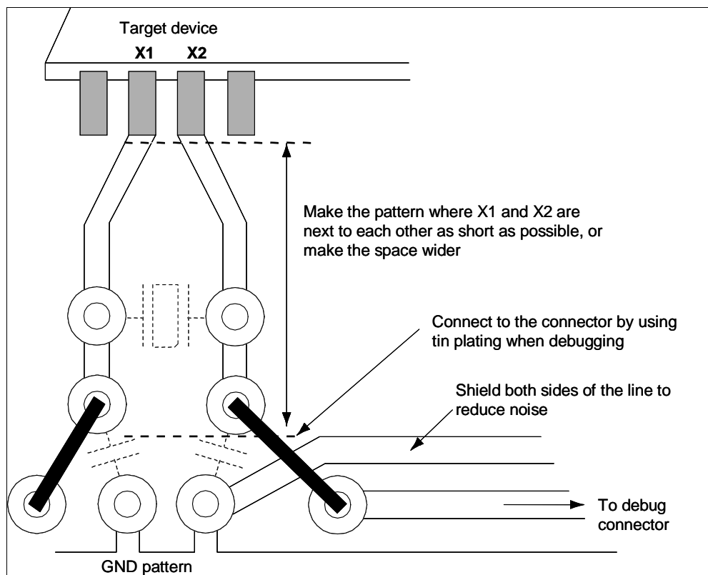
Figure 2-16. Reference Diagram of User System
