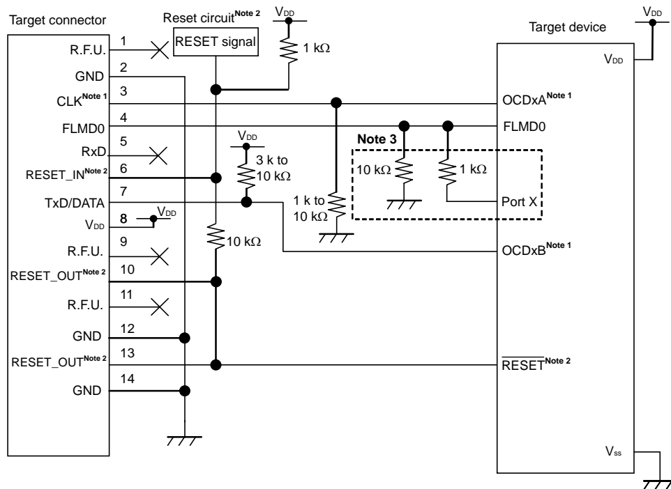
Figure 2-6. Only Debugging Is Performed (OCDxA, OCDxB Communication x = 0, 1)
