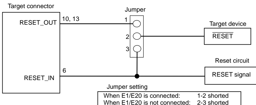
Figure 2-13. Circuit Connection for Switching Reset Signal with Jumper
