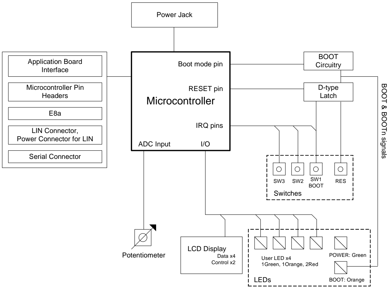
Figure 5-1: Block Diagram
