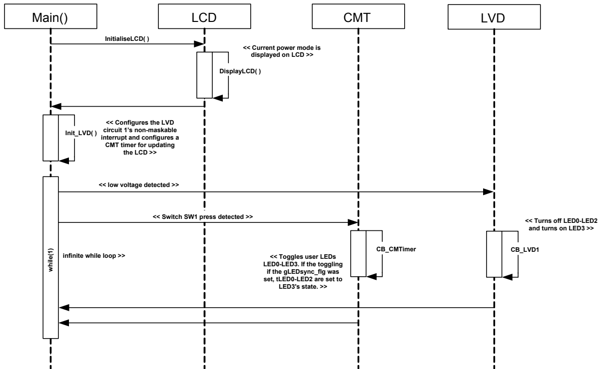
Figure 4-10: LVD Sequence Diagram
