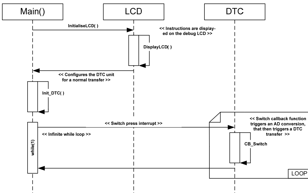
Figure 4-59: DTC Sequence Diagram
