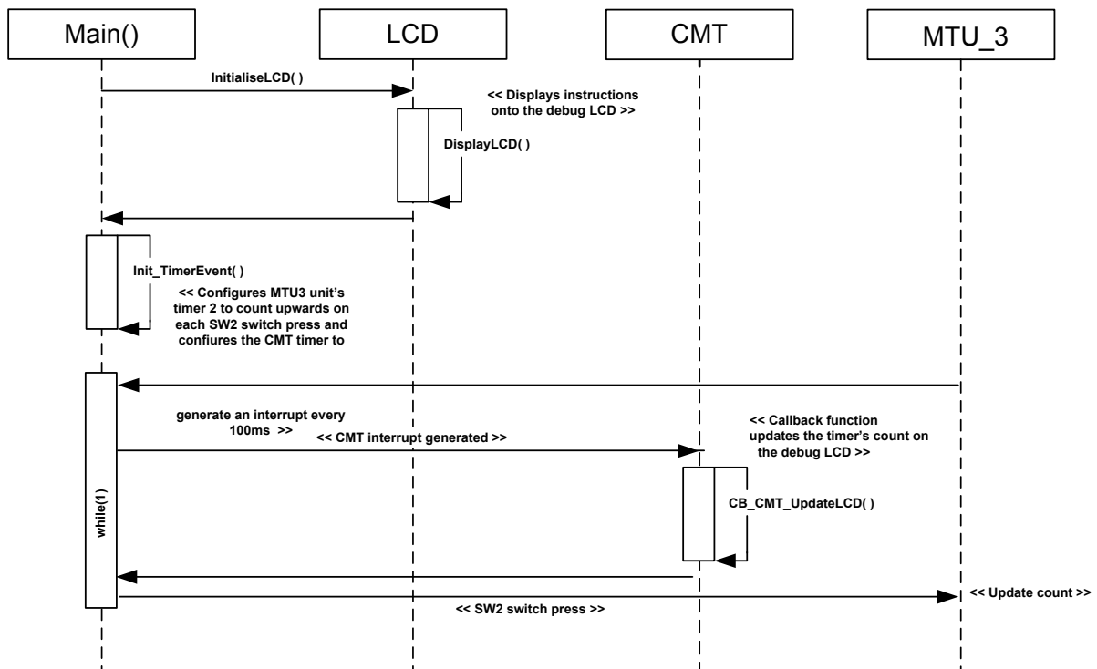
Figure 4-16: Timer_Event Sequence Diagram
