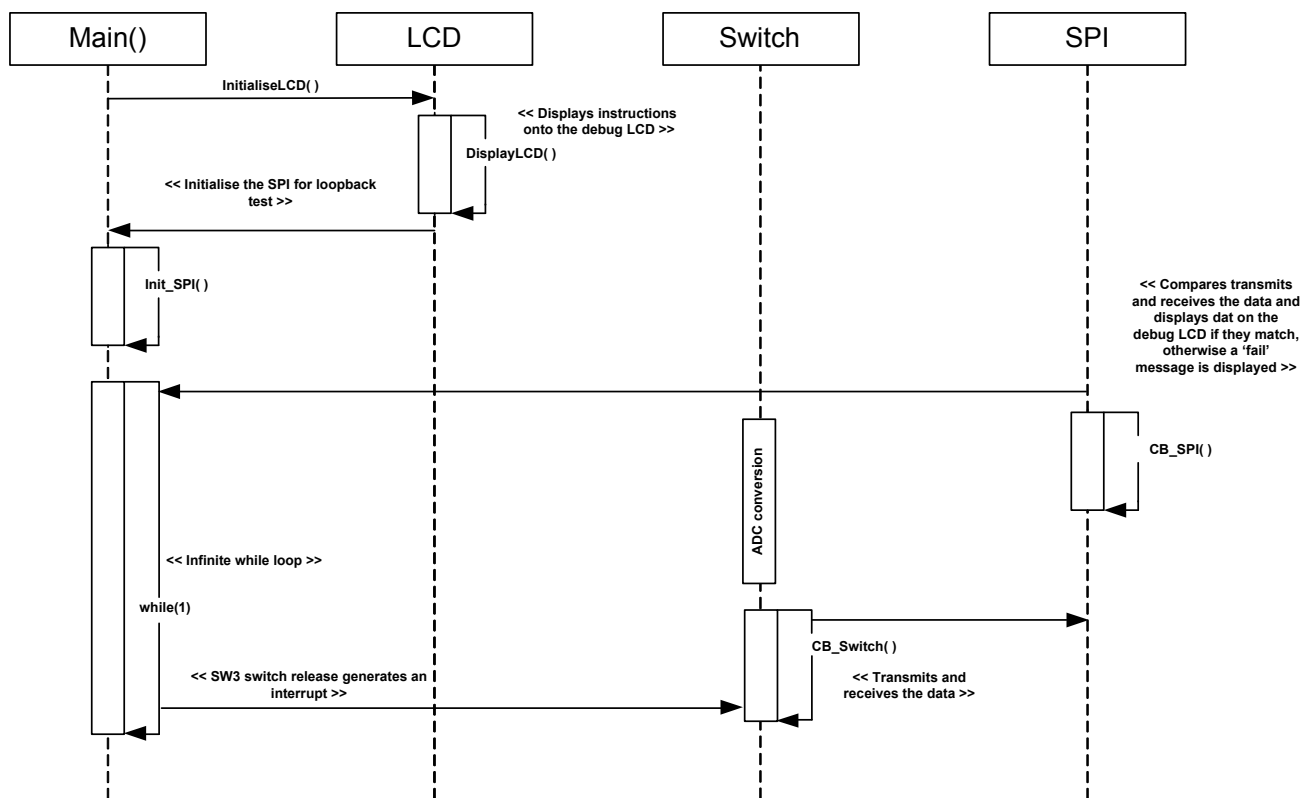
Figure 4-5: SPI Sequence Diagram
