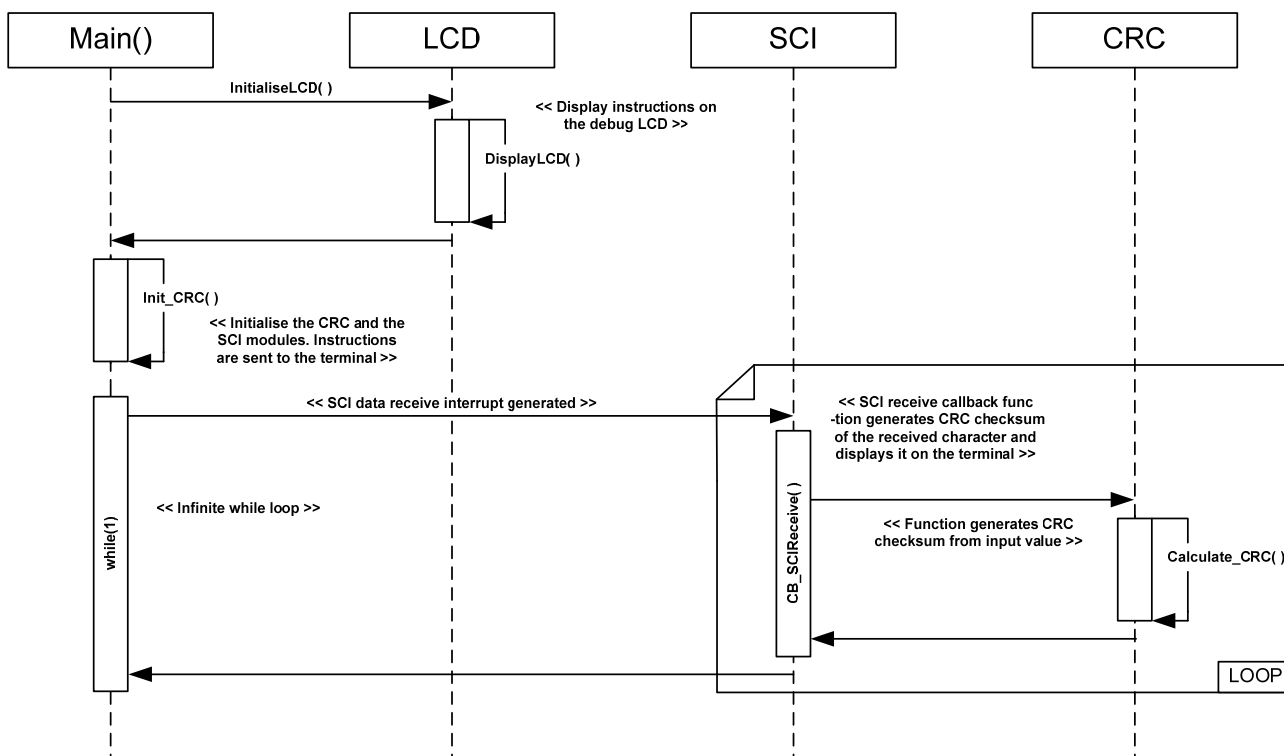
Figure 4-13: CRC Sequence Diagram
