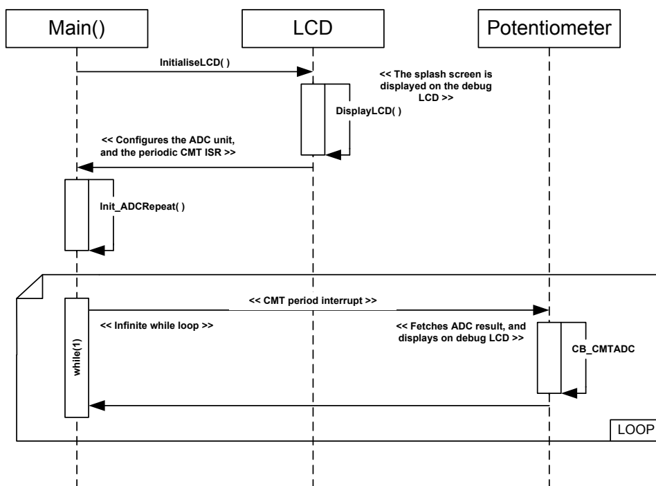
Figure 4-2: ADC_Repeat Sequence Diagram
