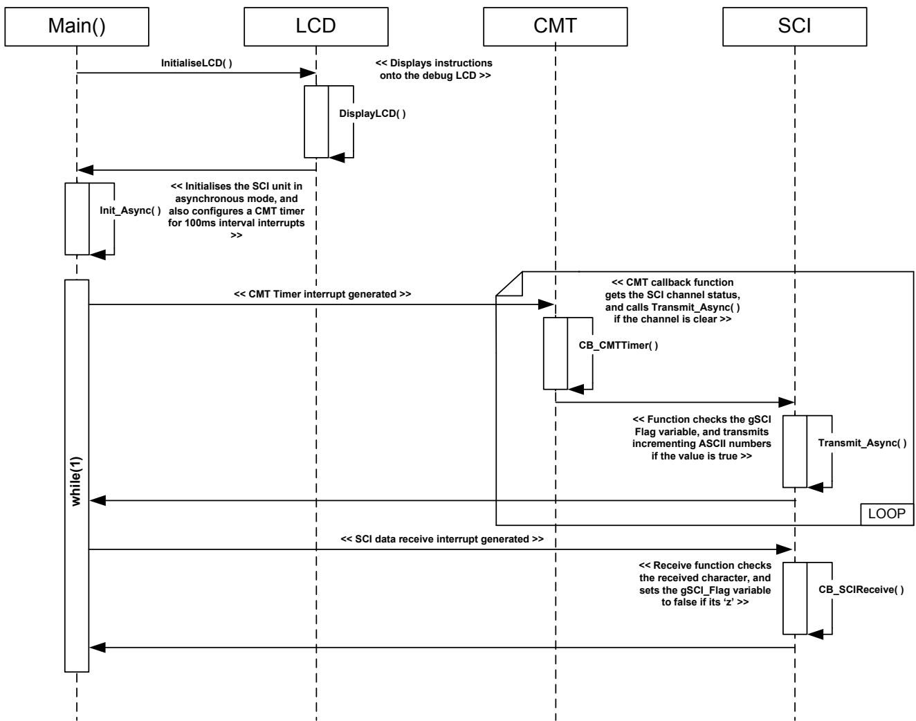
Figure 4-7: Async_Serial Sequence Diagram
