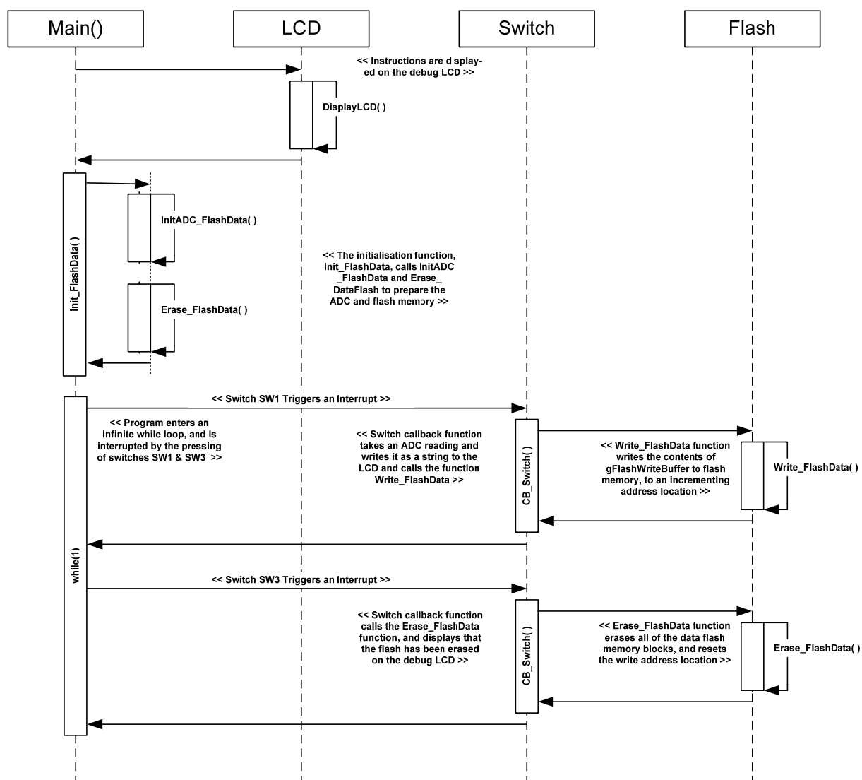
Figure 4-48: Flash_Data Sequence Diagram
