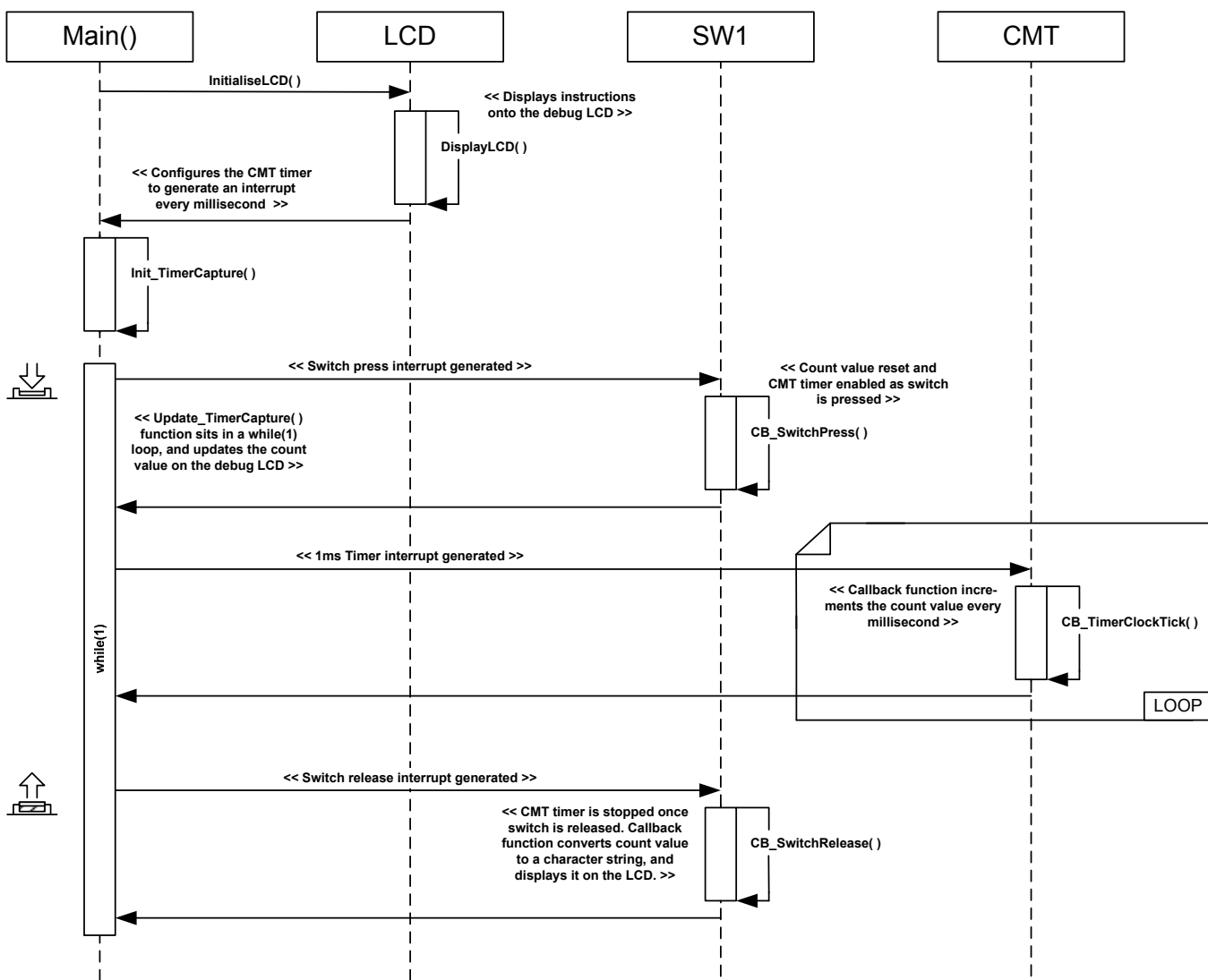
Figure 4-14: Timer_Capture Sequence Diagram
