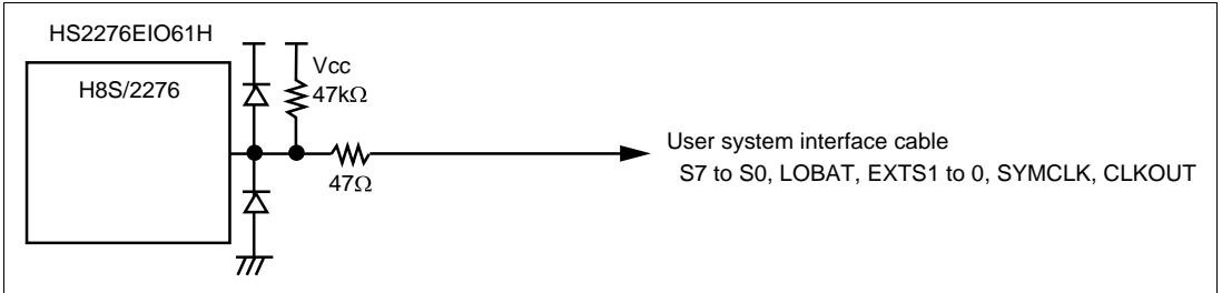
Figure 3.1 FLEX™ decoder Interface Signals
