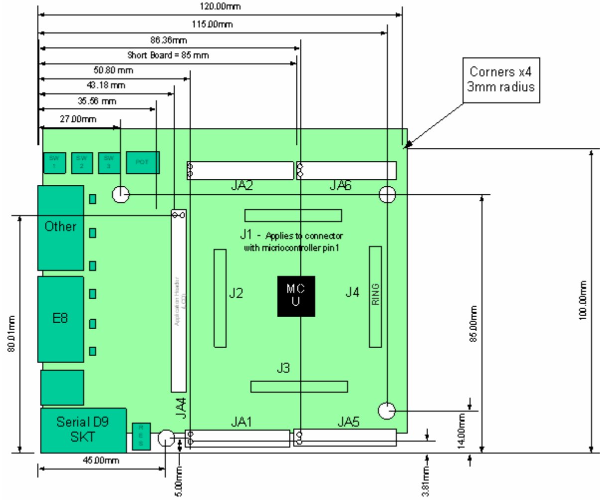
Figure 4-2 : Board Dimensions
