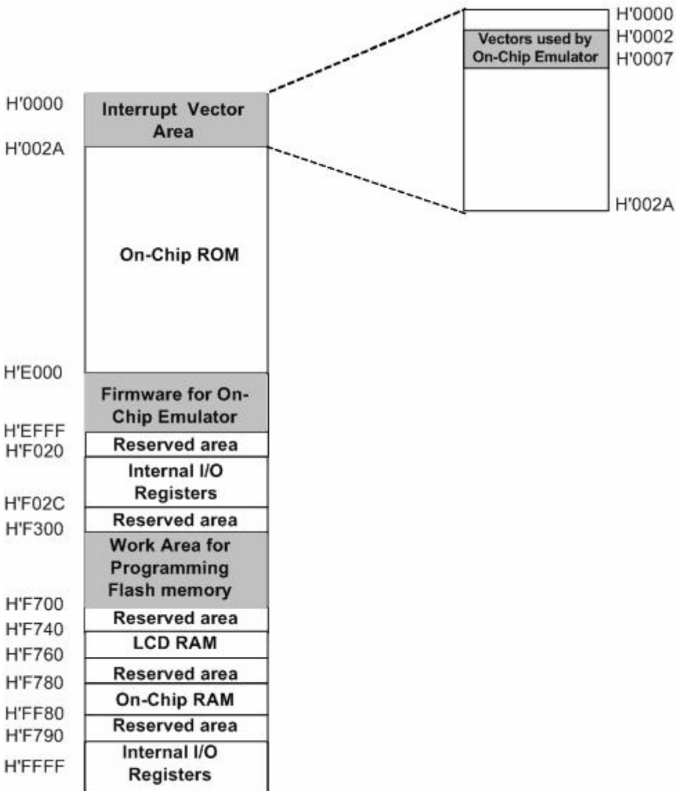
Figure 10-1: Memory Map
