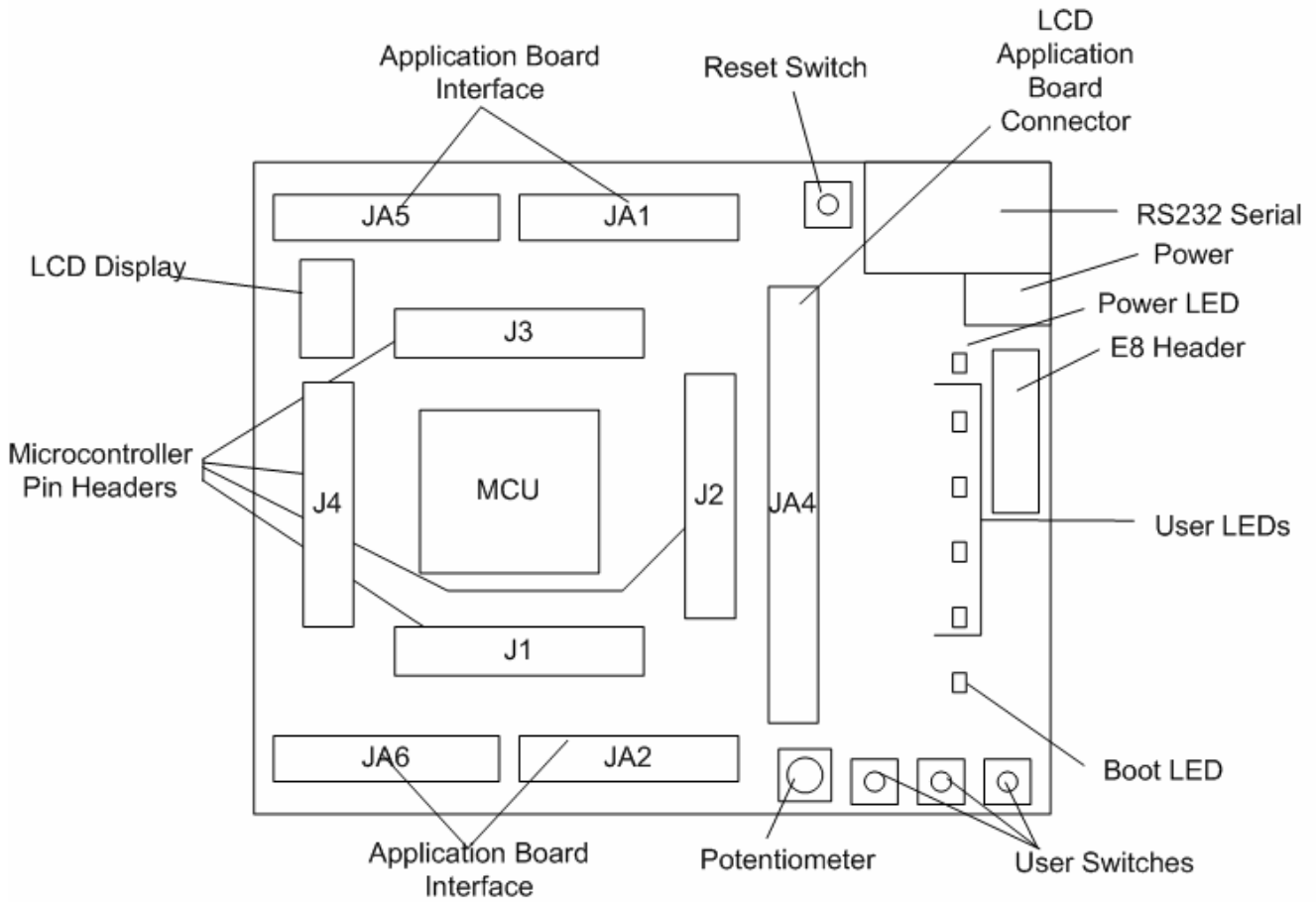
Figure 4-1: Board Layout
