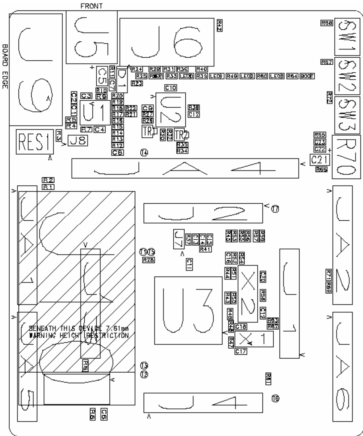
Figure 11-1: Component Placement
