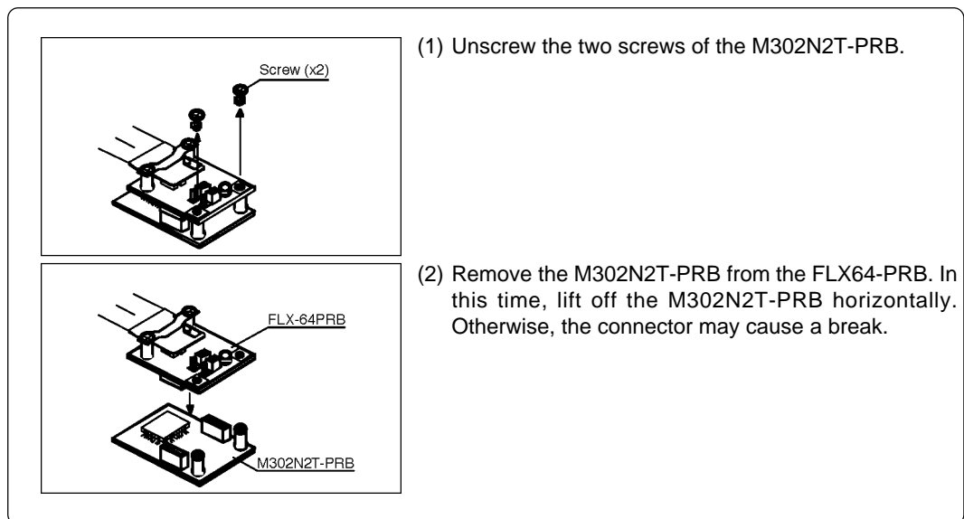
Figure 3.4 Removing pod probe M302N2T-PRB
