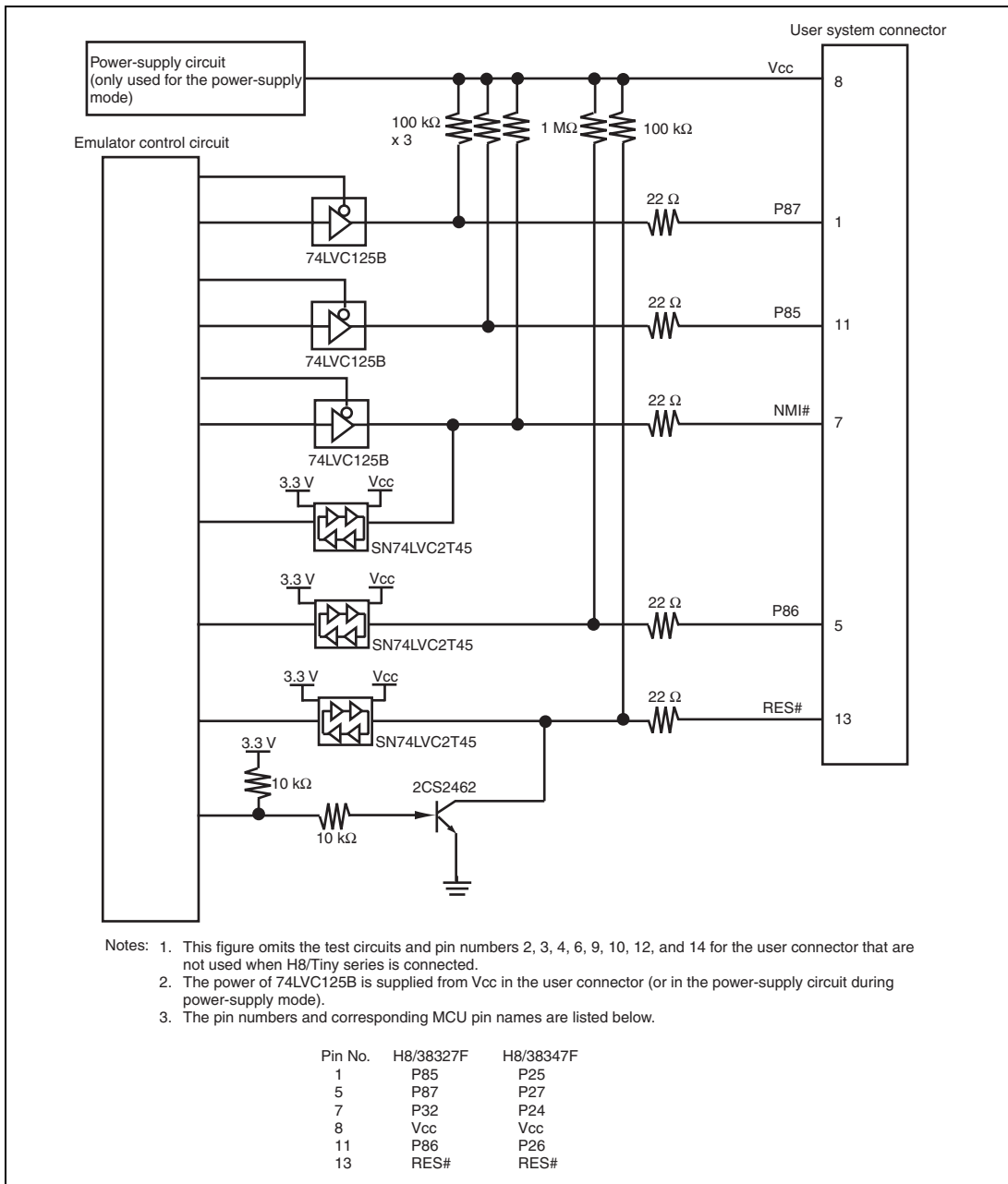
Figure 4.8 Interface Circuit in the E8a Emulator (Reference)
