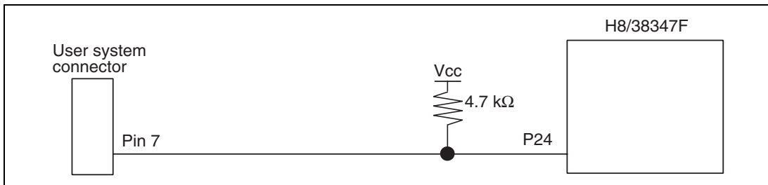
Figure 4.6 Connection of Emulator and P24 Pin (H8/38347F)
