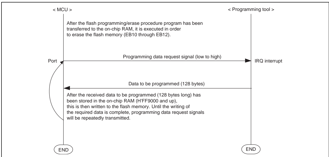
Figure 2 Control Operation
