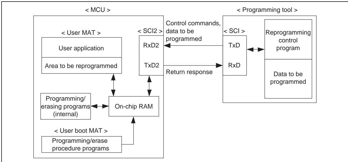
Figure 1 Block Diagram of On-Board Reprogramming using an SCI (asynchronous mode)
