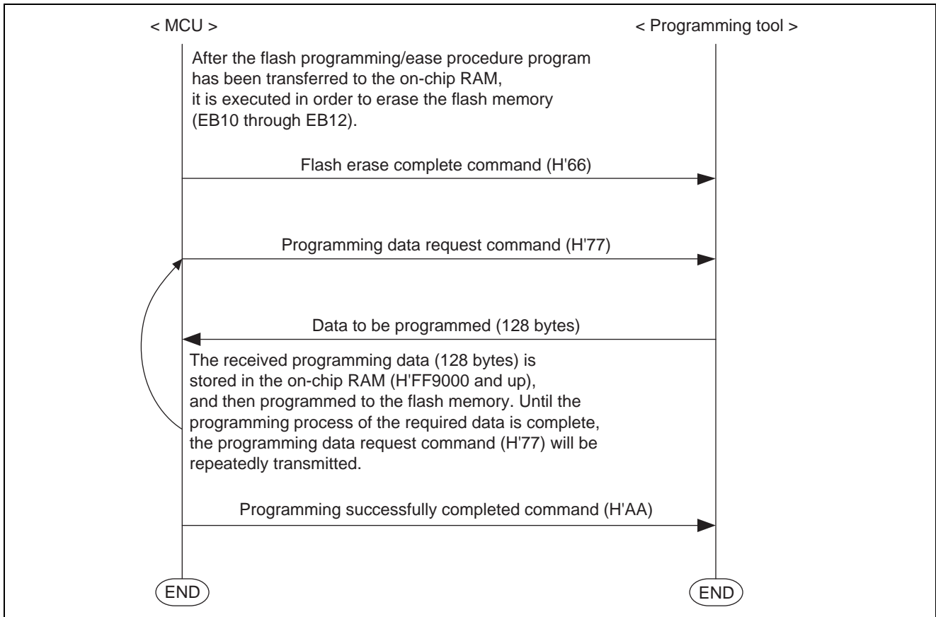
Figure 2 Control Command Behaviors
