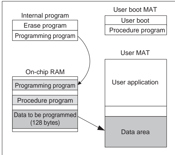
Figure 3 Description of Software Operation
