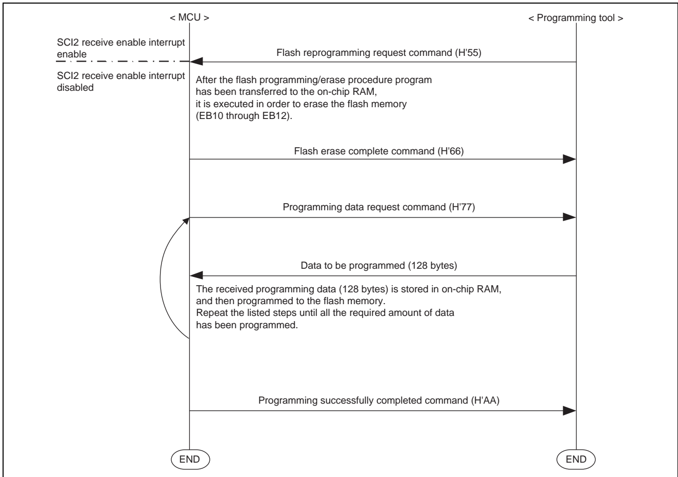
Figure 2 Control Command Behaviors
