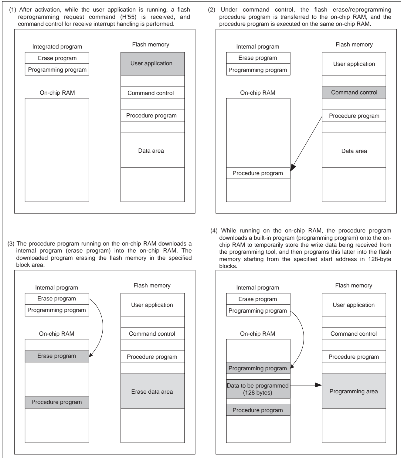
Figure 3 Description of Software Operation
