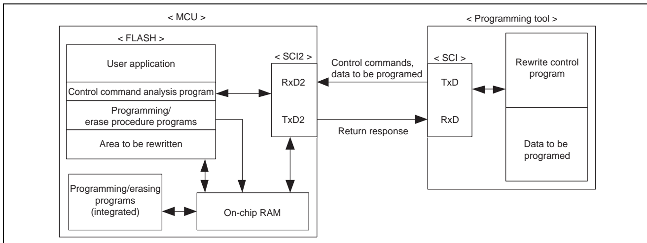
Figure 1 Block Diagram of On-Board Reprogramming Setup using an SCI (asynchronous mode)
