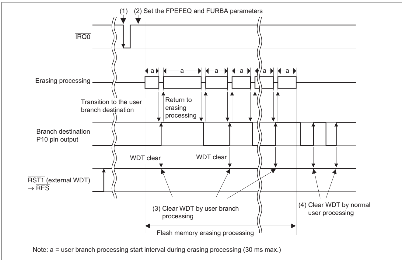
Figure 3 Operation Timing
