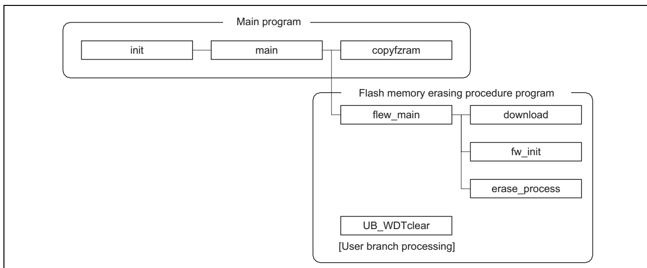
Figure 4 Hierarchical Structure
