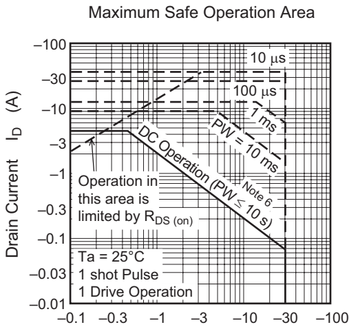
Drain to Source Voltage V_{DS} (V) Note 6: When using the glass epoxy board (FR4 40 × 40 × 1.6 mm)
